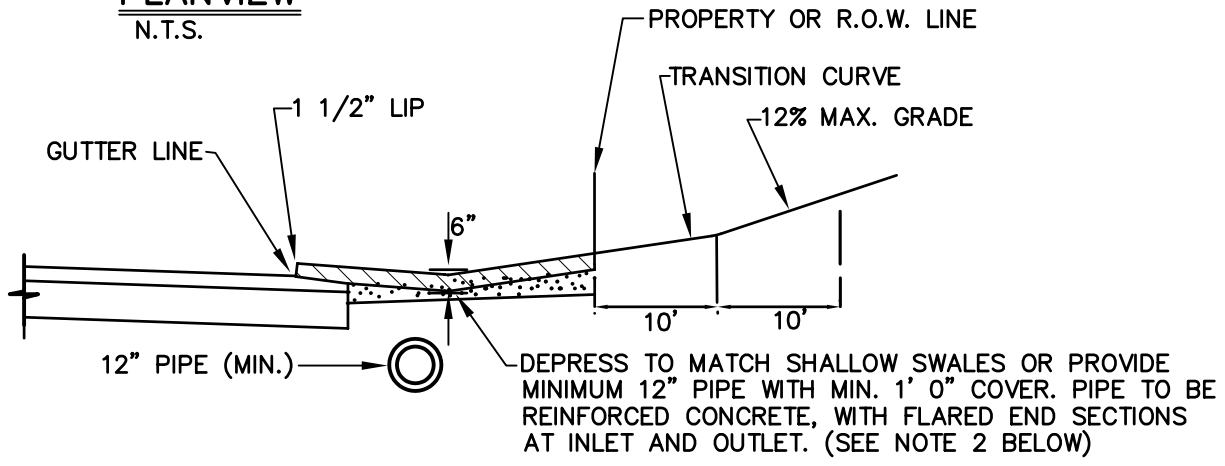
SECTION - UPHILL DRIVEWAY N.T.S.
