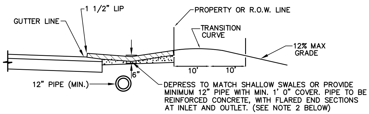
SECTION - DOWNHILL DRIVEWAY
